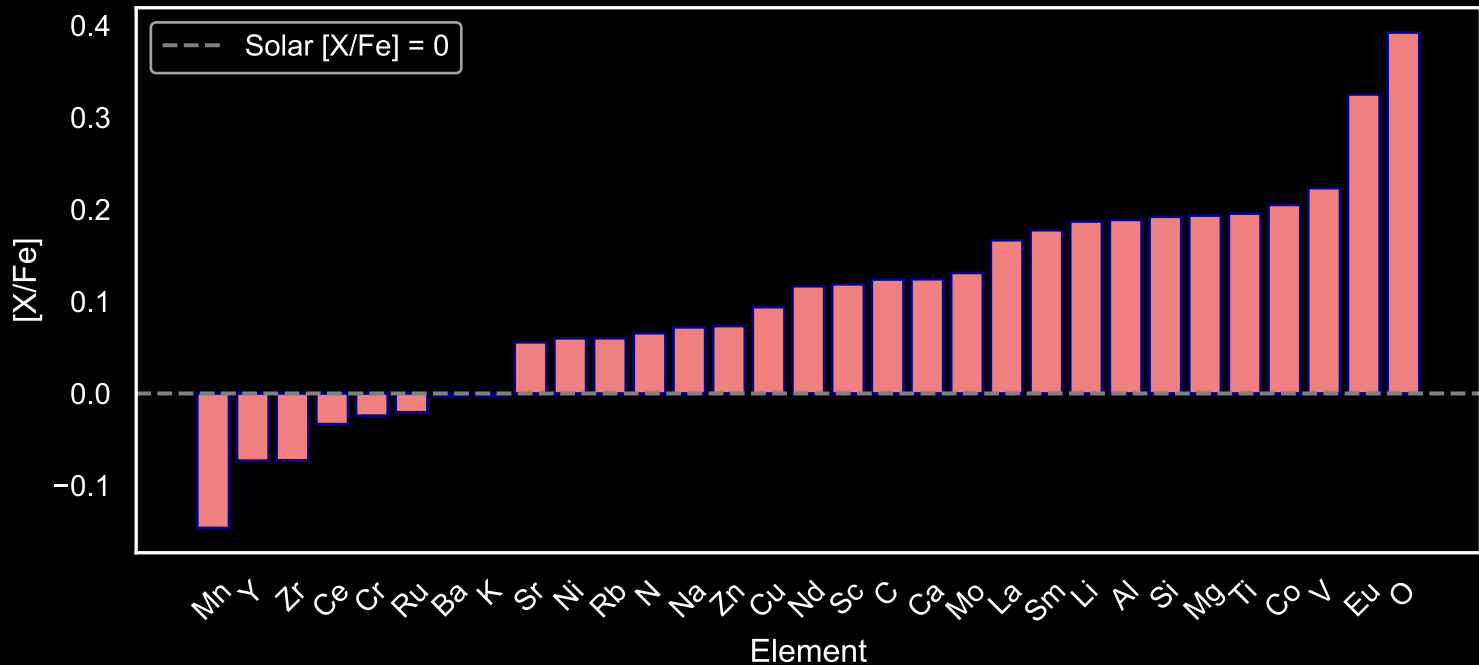
Abundance Pattern for GALAH Red Giants: Star Field [91] (N=47)
