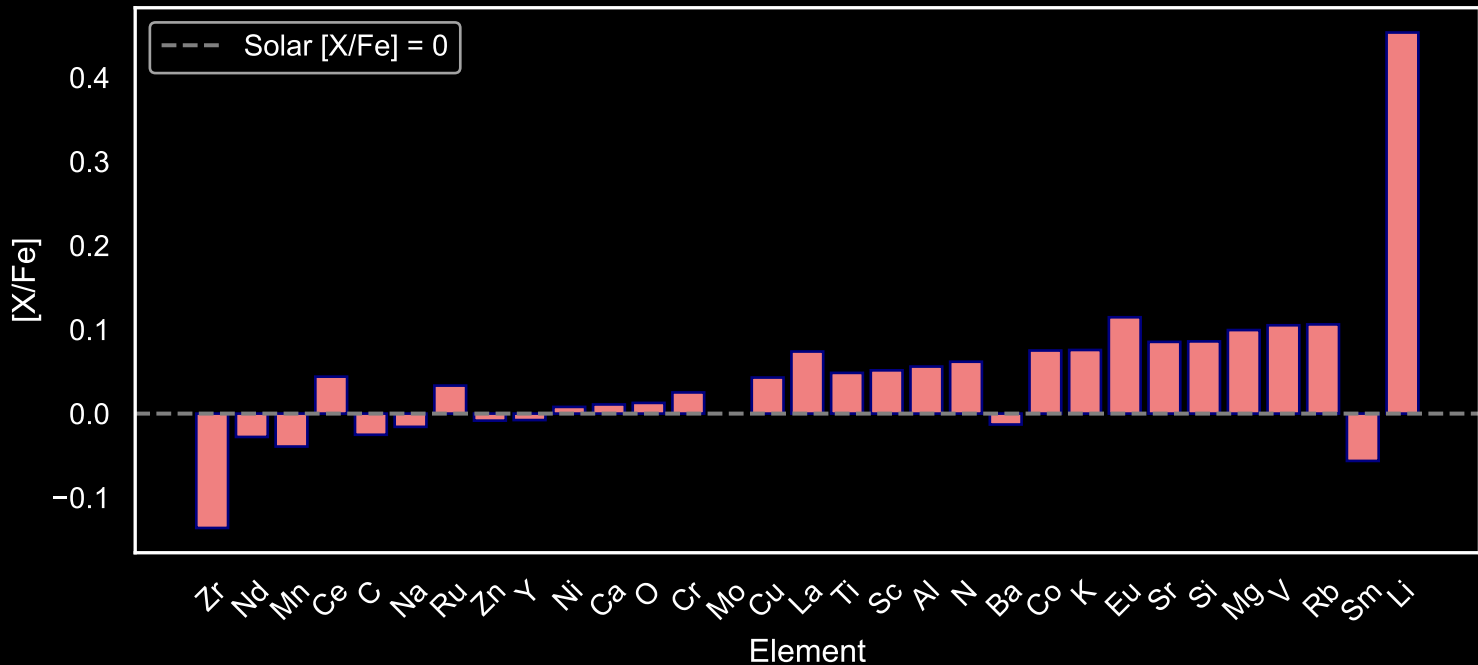
Abundance Pattern for GALAH Main Sequence Stars: Star Field [91] (N=111)
