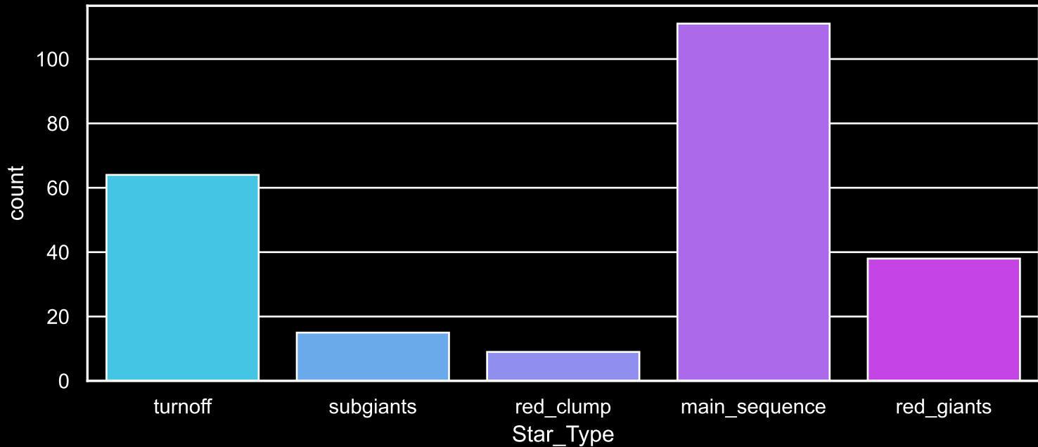
Field [91] Count plot of Star Type
