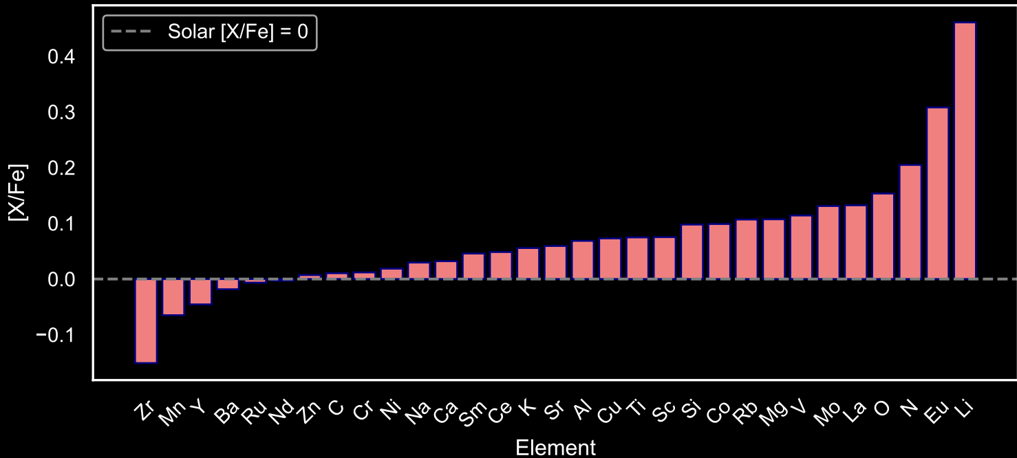
Abundance Pattern for GALAH Star Field [91] (N=237)
