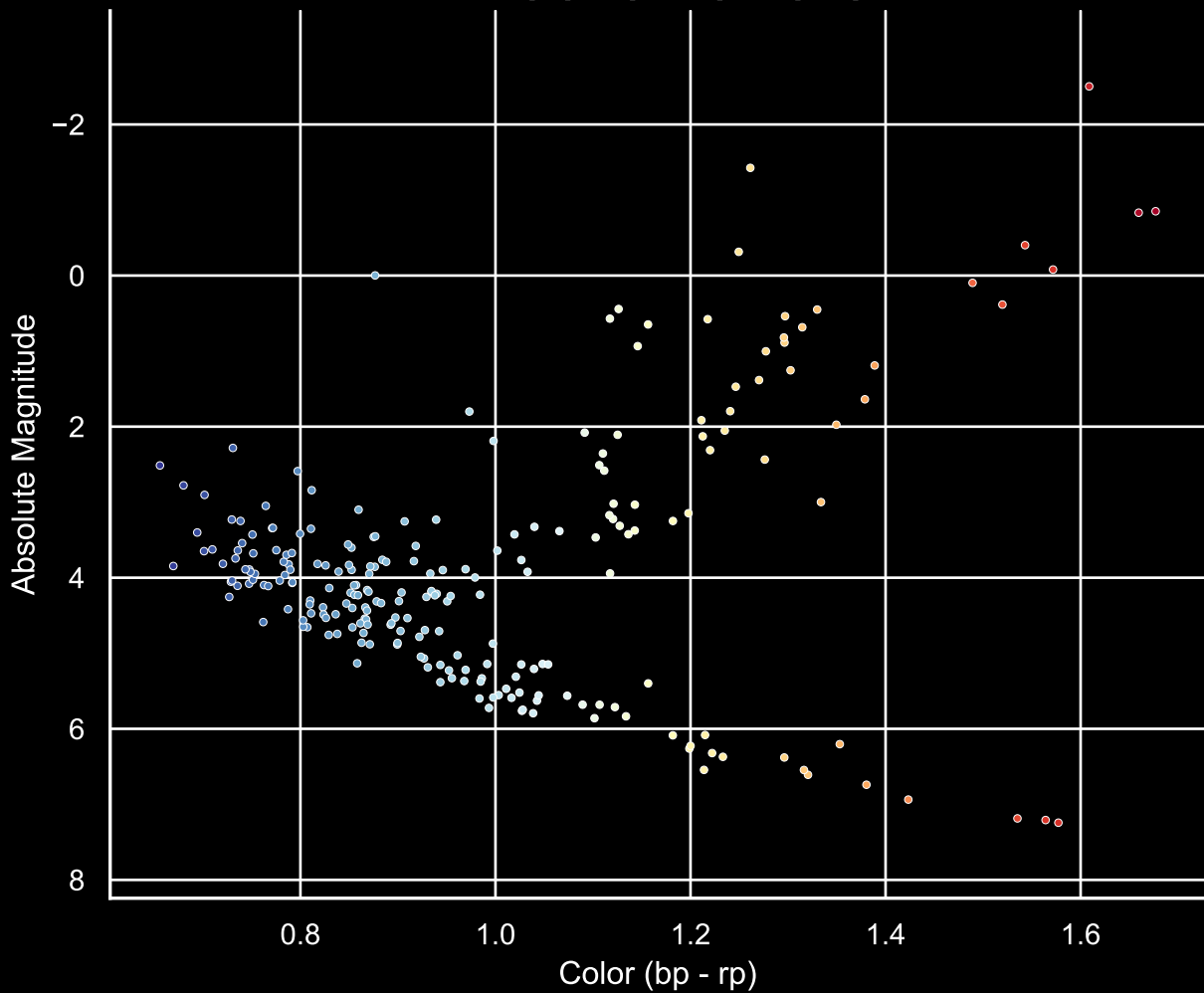
GALAH Hertzprung-Russel Diagram Field [91] Ra [335.02] Dec [1.57]
